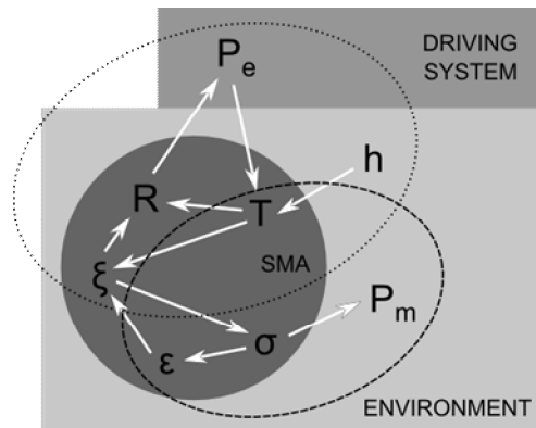
Figure 1. Schematic representation of an SMA based actuation system: in the three main areas the variables that influence the behavior of the alloy and their dependencies are depicted: the temperature, T , the electrical resistance, R , the deformation, \epsilon , and the stress, \sigma , the martensitic fraction, \xi , inside the alloy; the convection heat transfer coefficient, h , and the mechanical power acting on the environment, P_m ; the electrical power provided by the driving system, P_e .
