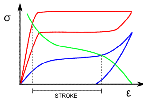
Figure 8. Stress vs. strain relationship of a SMA in martensite (blue) and austenite (red) phase that acts against an elastomer (green). The intersection points among the curves dictate the maximum available stroke that the system can implement.
