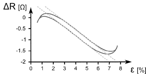
Figure 9. Resistance vs. strain curve. Due to the low hysteresis the linearized function can be used in the control loop.
