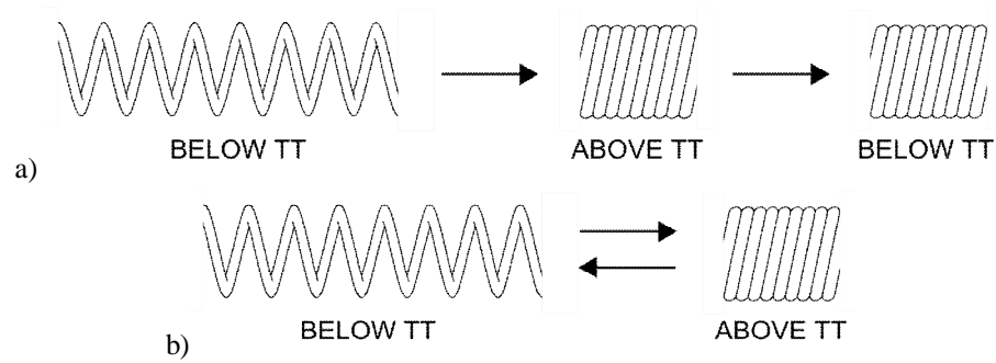
Figure 2. Spring showing the SME: after apparent permanent deformation induced below the TT the alloy can recover the initial shape by heating above the TT; after temperature drop OWE (a) or TWE (b) can be observed.
