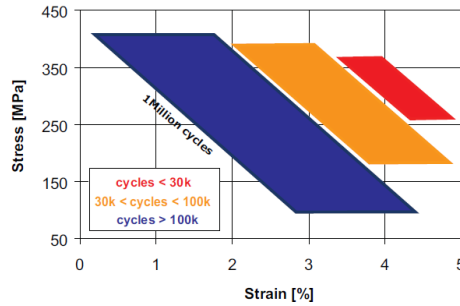
Figure 7. Diagram required to assess the stress-strain tradeoff depending on the expected actuator life. (source: SAES Getters)
