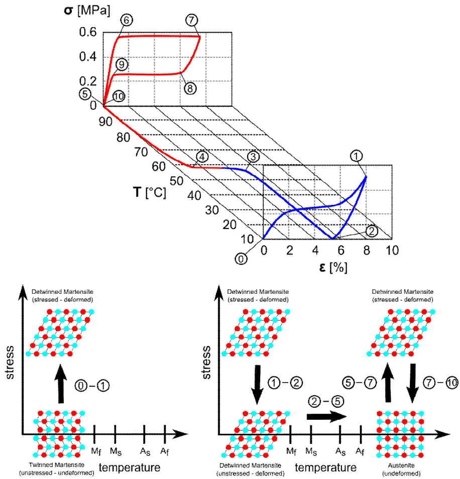
Figure 6. Thermo-mechanical behavior of a SMA showing the dependency among temperature, T , stress, \sigma , and strain, \epsilon , and the related crystal structures.
