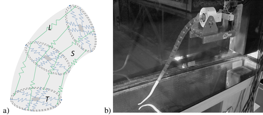
Figure 10. Schematic design of the artificial muscular hydrostats (a), with 4 longitudinal SMA actuators (L), a number of transverse SMA actuators (T) and the support structure (S); entire octopus-like arm (b).
