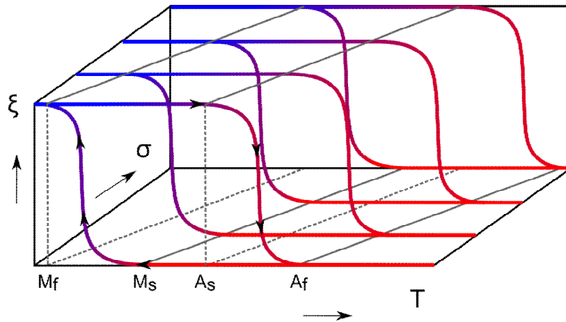
Figure 5. Diagram showing martensite fraction, \xi , versus temperature, T , relationship at constant loads, \sigma . Thermodynamic cycles are shifted rightwards (stress gradient) increasing the transformation temperature values.
