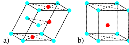
Figure 4. Crystal structure of martensite (a) and austenite (b).
